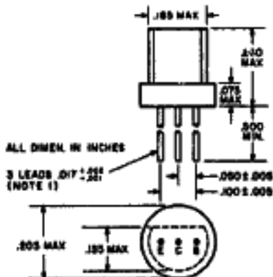
TO-98
