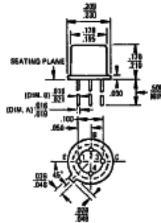
TO-72
