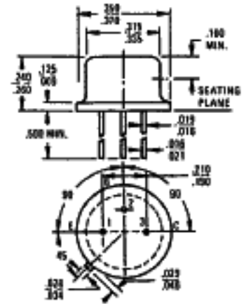
TO-39
