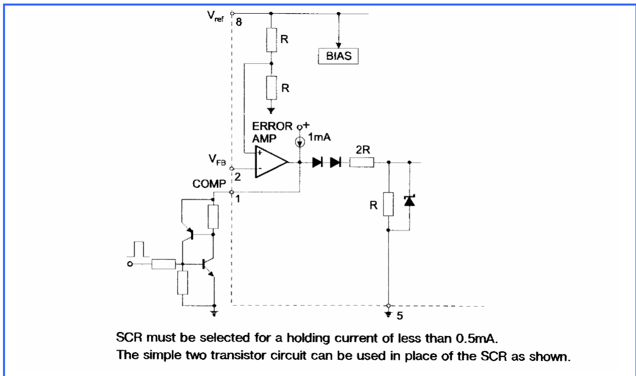
Figure 5:Latched Shutdown
