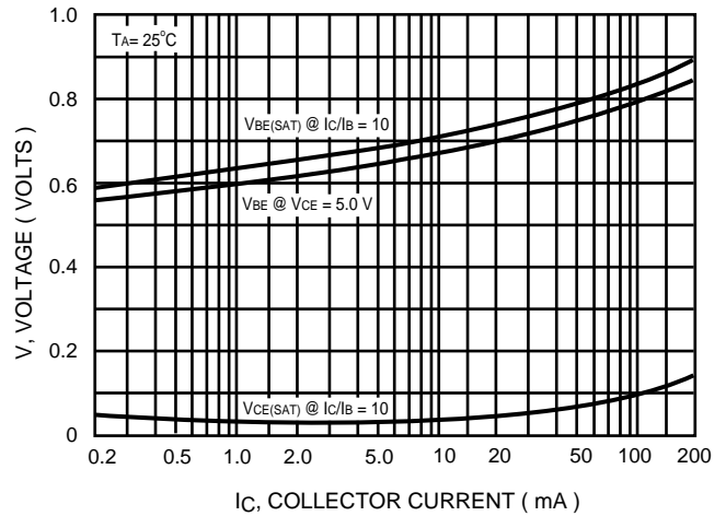
Figure 8. "On" Voltage
