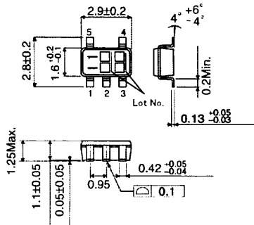
BU4S11G2(SSOP5)(UNIT:[mm])
