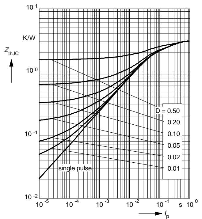
Transient thermal impedance Diode Z_{th\text{JC}} = f(t_p) parameter: D = t_p / T
