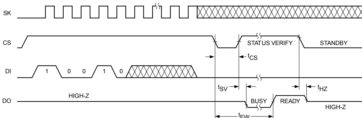
Figure 8. ERL Instruction Timing
