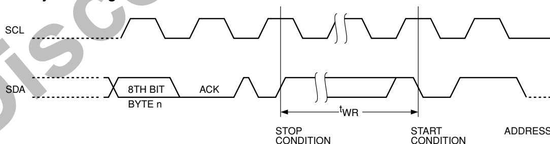
Figure 3. Start/Stop Timing
