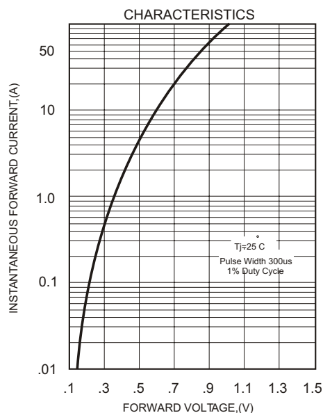
FIG.2-TYPICAL FORWARD CHARACTERISTICS
