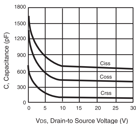
Figure 3. Capacitance
