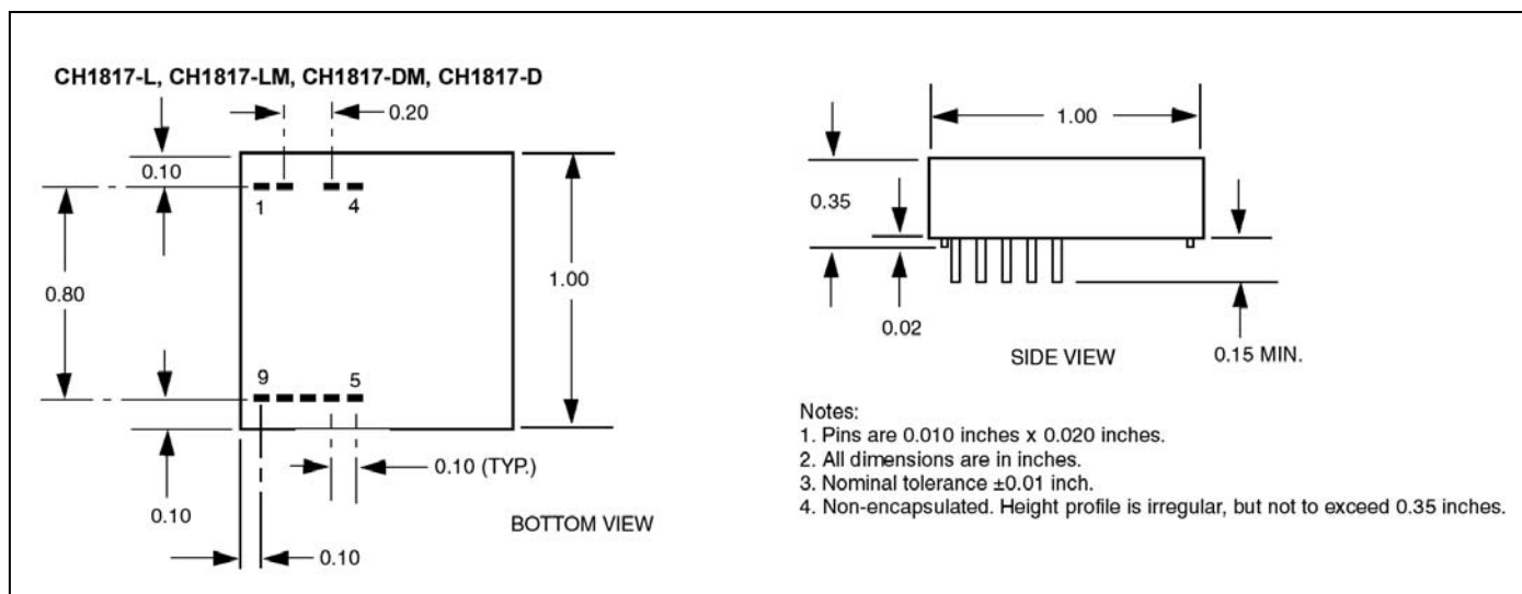
Figure 7. Mechanical Specifications.
