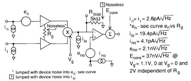
Figure 4: CLC520 Noise Model
