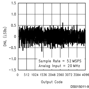
Differential Non-Linearity
