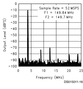
Two Tone Output Spectrum
