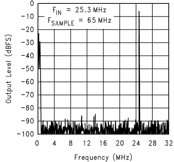
Spectral Response
