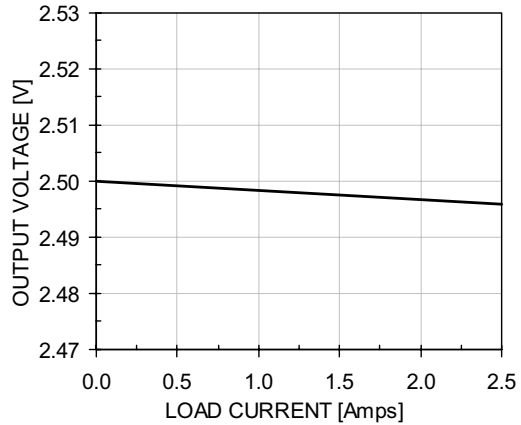
Load Regulation
