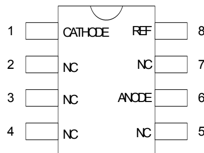
SOP-8 Top View
