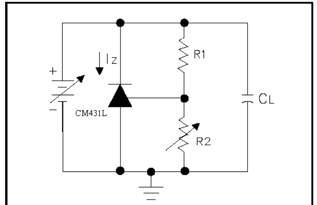
Stability Circuit
