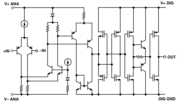
Figure 1. Simplified Schematic
