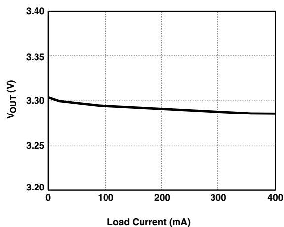
Figure 3. Load Regulation
