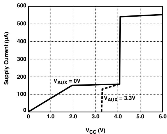
Figure 1. Supply Current vs Voltage ( V_{AUX} = 3.3V )
