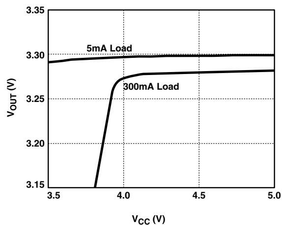
Figure 4. Line Regulation
