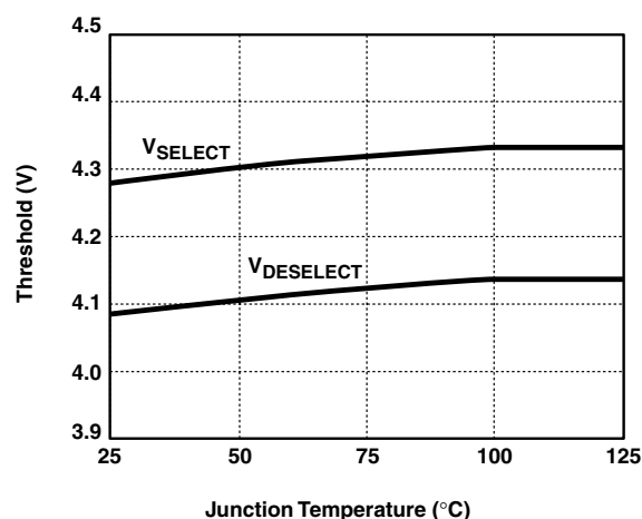
Figure 12. Select and Deselect Threshold vs T_{JUNC}
