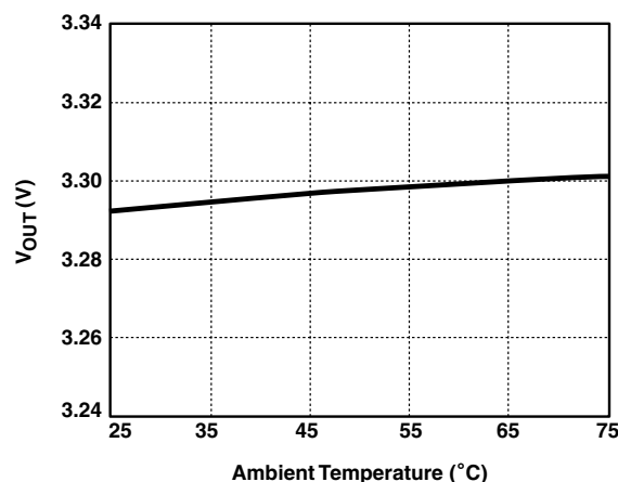
Figure 11. Regulator V_{OUT} vs T_{AMB} (300mA Load)
