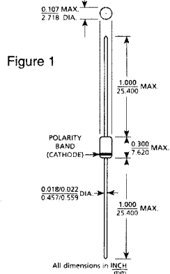
Package Drawing
