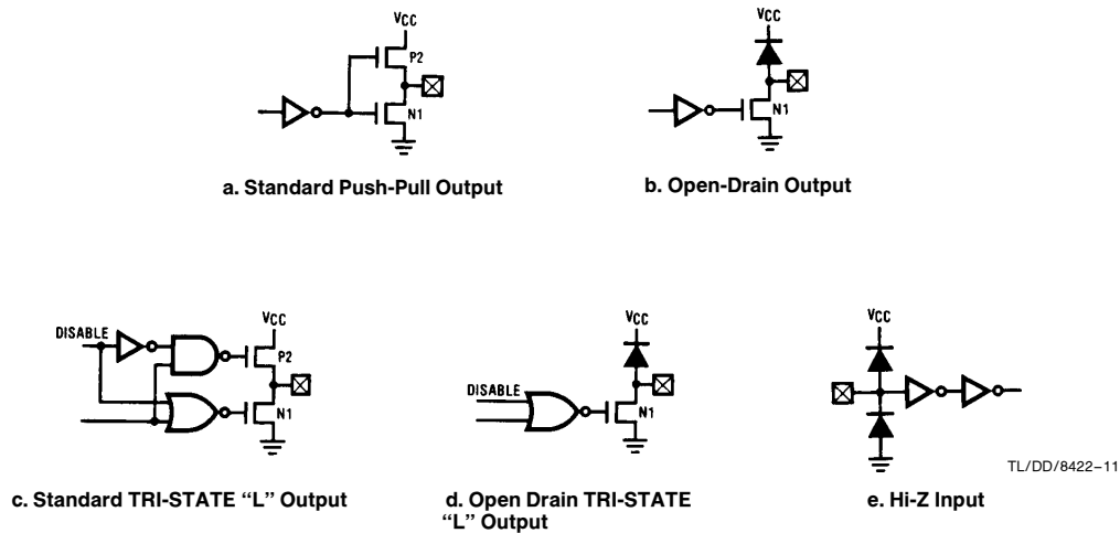
FIGURE 8. Input/Output Configurations
