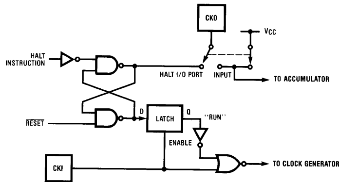
FIGURE 6b. Halt Mode—One-Pin Oscillator
