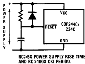
FIGURE 4. Power-Up Circuit
