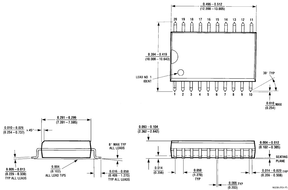
20-Lead Surface Mount Package (M) Order Number COP226C-XXX/WM NS Package Number M20B
