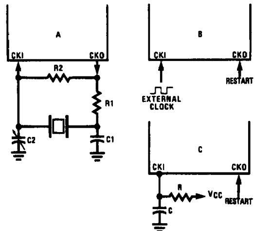
FIGURE 6. Crystal and R-C Connection Diagrams
