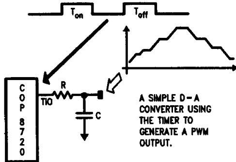
FIGURE 12. Timer Application
