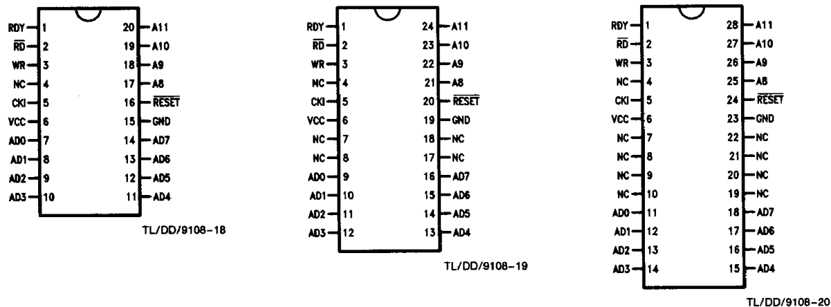
FIGURE 4. Pinouts for the COP8720C in Programming Mode
