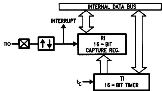
FIGURE 11. Timer Capture Mode Block Diagram
