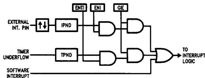
FIGURE 7. Interrupt Block Diagram
