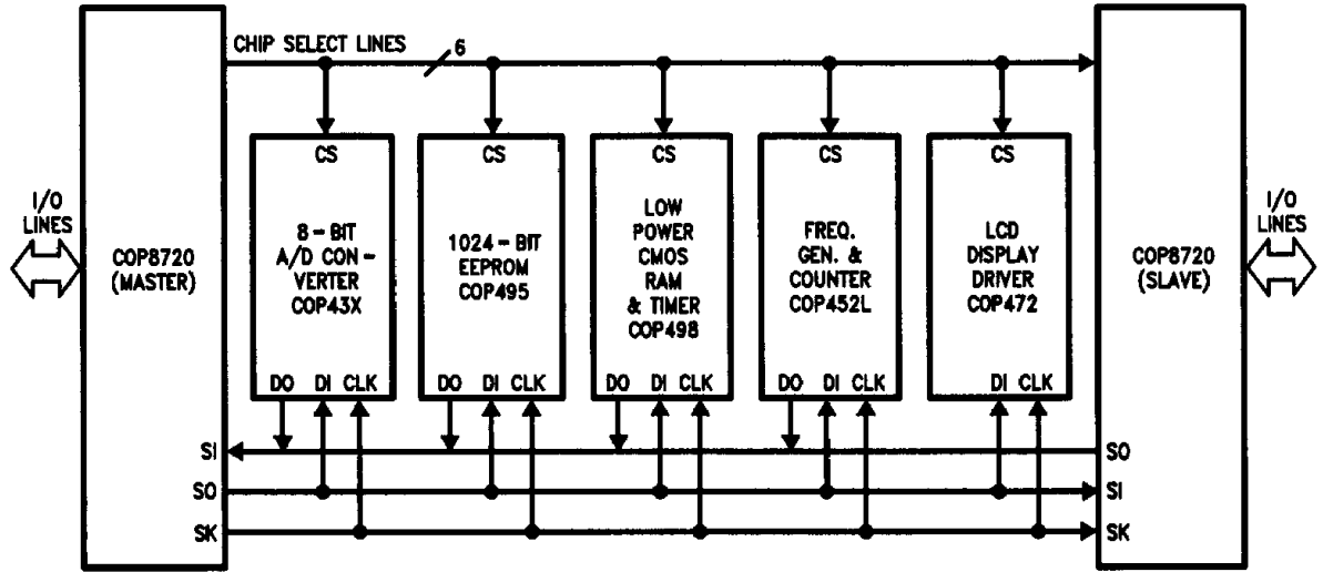
FIGURE 9. MICROWIRE/PLUS Application
