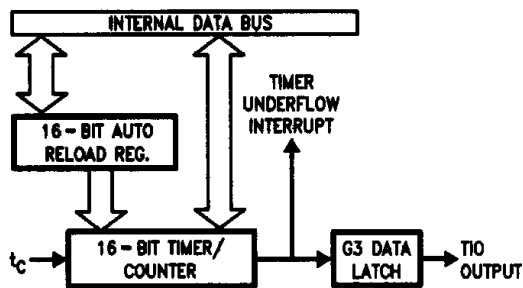
FIGURE 10. Timer/Counter Auto Reload Mode Block Diagram
