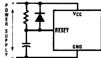
RC ≥ 5X Power Supply Rise Time FIGURE 5. Recommended Reset Circuit
