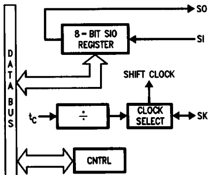
FIGURE 8. MICROWIRE/PLUS Block Diagram
