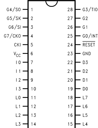
28 DIP
