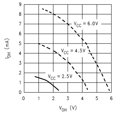
Port L/G Push-Pull Source Current
