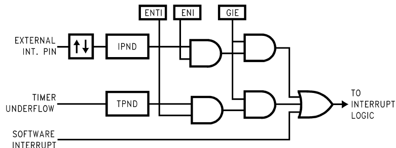
FIGURE 5. Interrupt Block Diagram
