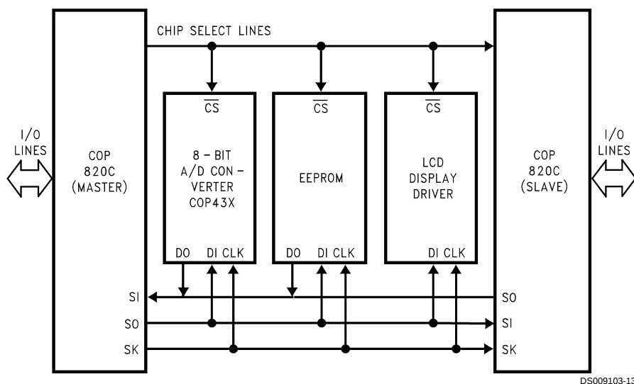
FIGURE 7. MICROWIRE/PLUS Application
