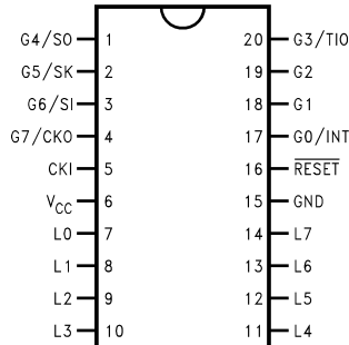
DUAL-IN-LINE PACKAGE 20 DIP
