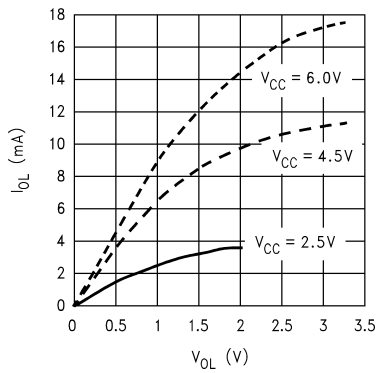
Port L/G Push-Pull Sink Current
