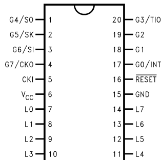
SURFACE MOUNT 20 SO Wide
