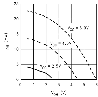
Port D Source Current
