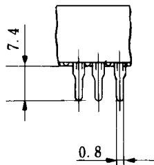
(2) Through hole
