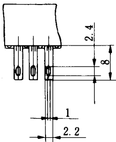
(1) Eyelet
