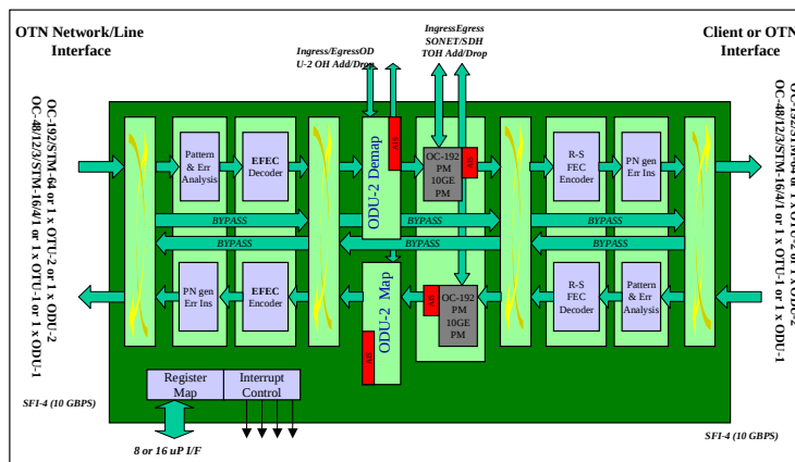
Figure 1: Block Diagram
