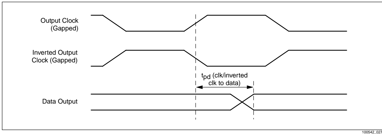
Figure 4-6. System-Side Receiver Interface Timing
