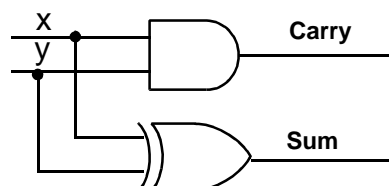
Figure 4. One-Bit Half Adder
