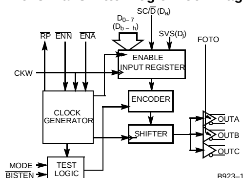
CY7B923 Transmitter Logic Block Diagram
