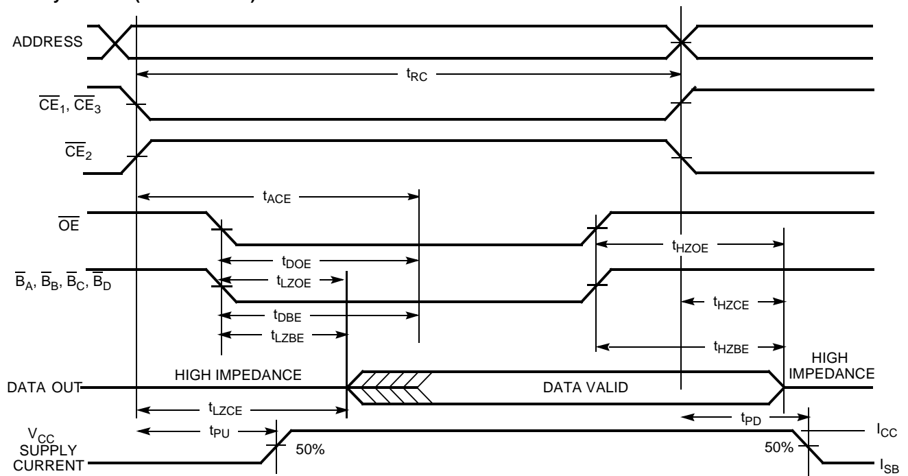
Read Cycle No. 2 (OE Controlled) [11, 12]
