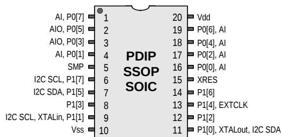
CY8C24223 20-Pin PSoC Device
