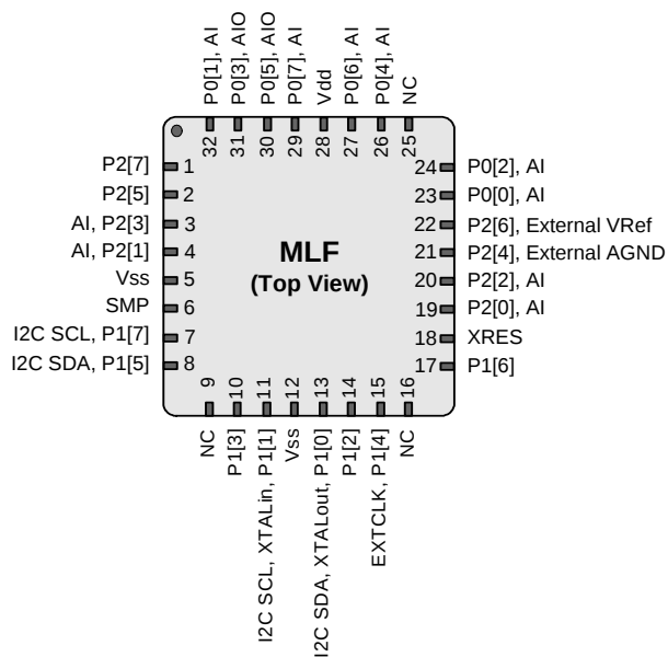
CY8C24423 PSoC Device
