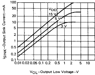
OUTPUT SINK CURRENT
