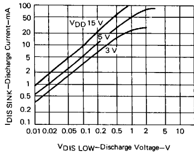
DISCHARGE CURRENT
