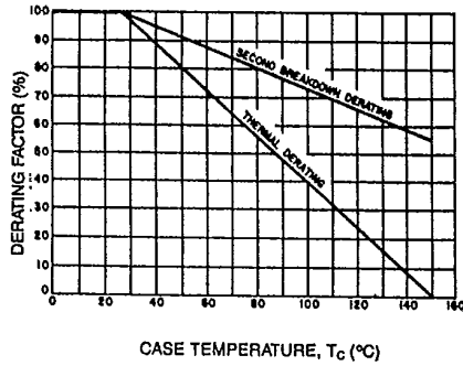
DERATING FACTOR OF SAFE OPERATING AREA (S.O.A.)
