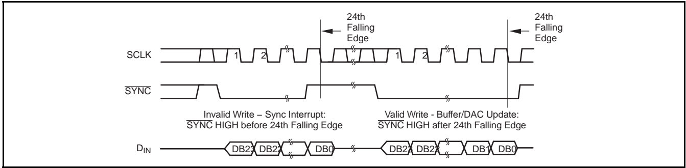
Figure 44. Interrupt and Valid \overline{\text{SYNC}} Timing
