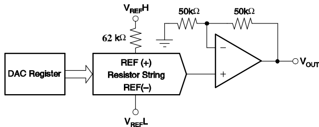
Figure 47. DAC8555 Architecture
