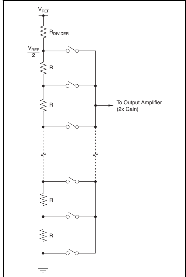
Figure 63. Resistor String
