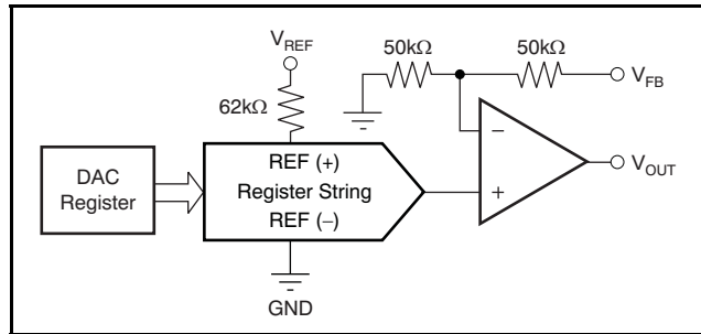
Figure 62. DAC8560 Architecture
