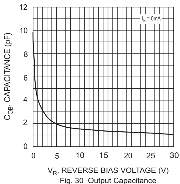
Fig. 30 Output Capacitance
