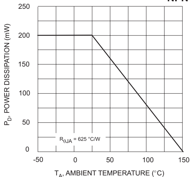
Fig. 33 Derating Curve
