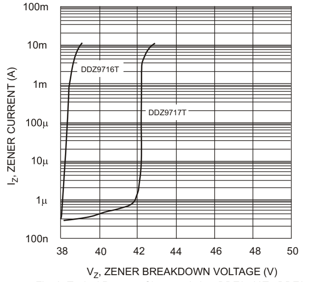
Fig. 9 Typical Reverse Characteristics, DDZ9716T - DDZ9717T
