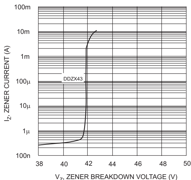
Fig. 9 Typical Reverse Characteristics, DDZX43
