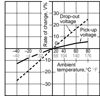
5.-(1) Ambient temperature characteristics (1 Form A) Tested sample: DE1a-5V, Ambient temperature: -40°C to 80°C -40°F to 176°F, Quantity: n=6
