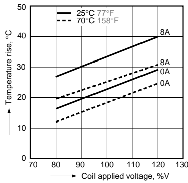
3.-(3) Coil temperature rise (2 Form A) Tested sample: DE2a-5V Quantity: n=6 Ambient temperature: 25°C to 70°C 77°F to 158°F
