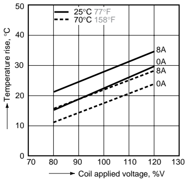
3.-(2) Coil temperature rise (1 Form A 1 Form B) Tested sample: DE1a1b-5V Quantity: n=6 Ambient temperature: 25°C to 70°C 77°F to 158°F
