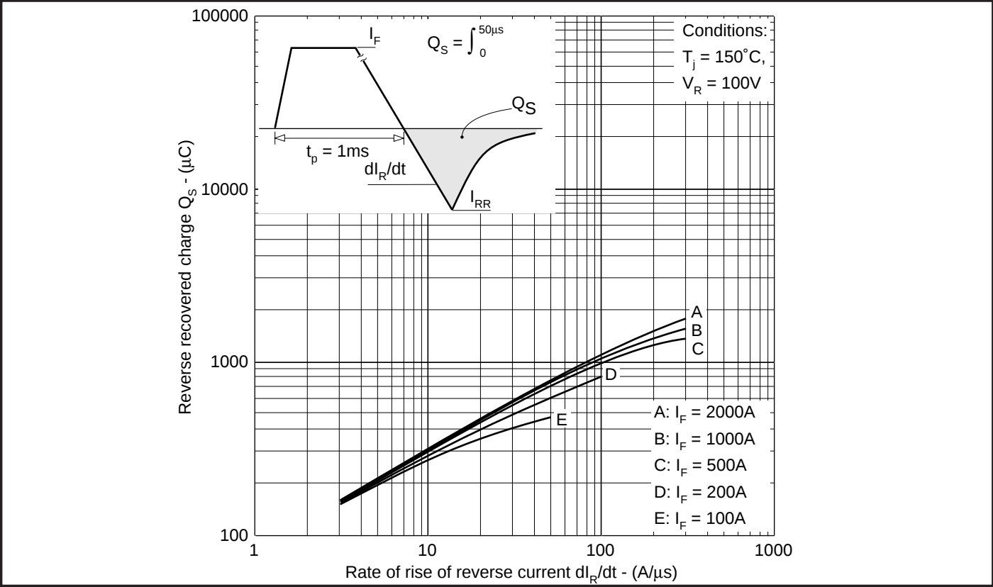
Fig.3 Recovered charge
