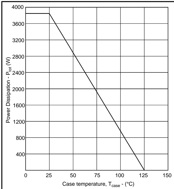
Fig. 5 Power dissipation
