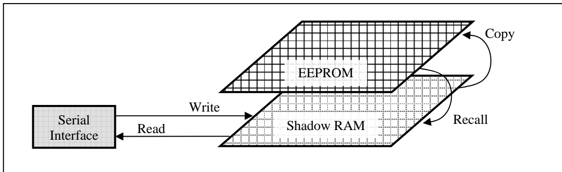
Figure 21. EEPROM Access via Shadow RAM
