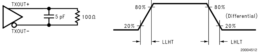
FIGURE 3. DS90C2501 (Transmitter) LVDS Output Load and Transition Times
