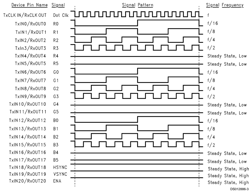
FIGURE 2. "16 Grayscale" Test Pattern (Notes 6, 7, 8, 9)
