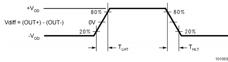
FIGURE 5. LVDS Output Transition Time
