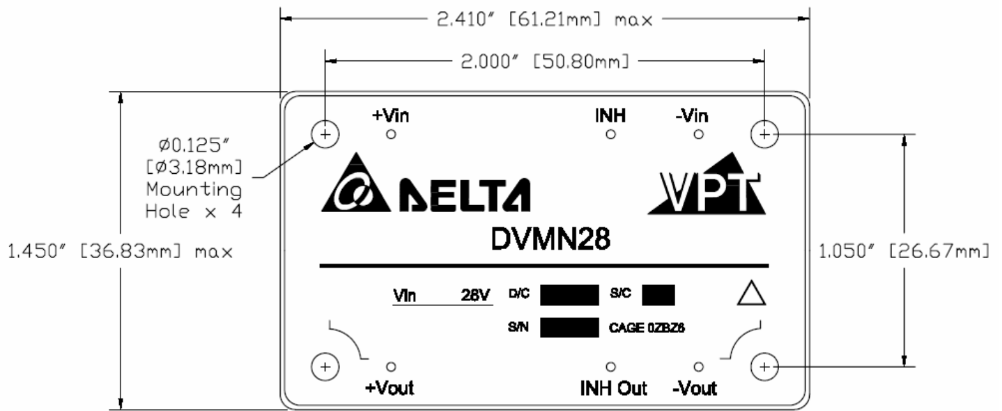
TOP VIEW
