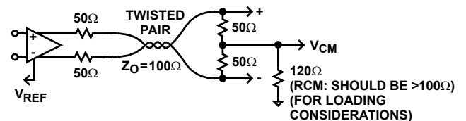
FIGURE 38. TWISTED PAIR TERMINATION EL4543
