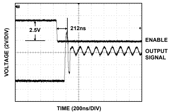
FIGURE 12. ENABLE RESPONSE
