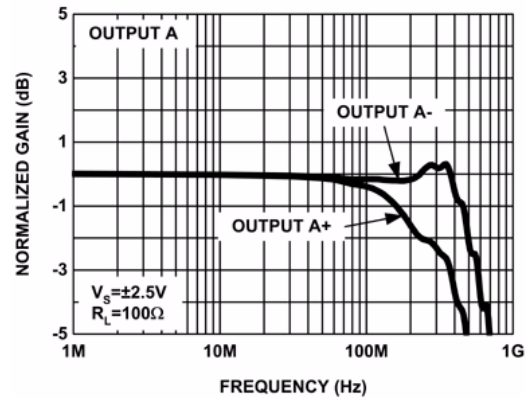
FIGURE 24. GAIN vs FREQUENCY - 2 CHANNELS
