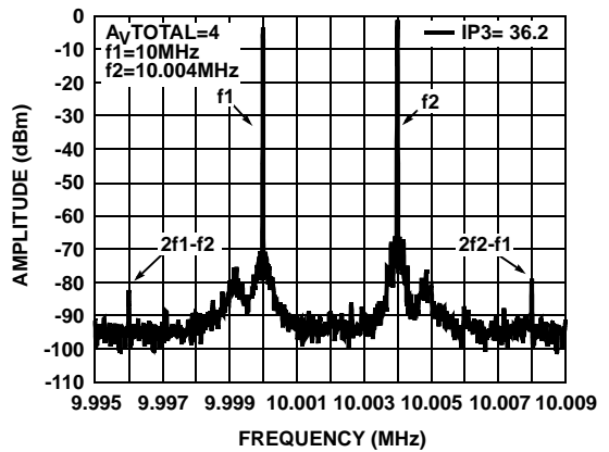
FIGURE 42. IP3 A_{vTOTAL} = 4 BLUE CHANNEL
