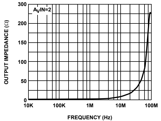
FIGURE 22. OUTPUT IMPEDANCE
