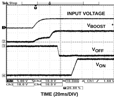
FIGURE 13. START-UP SEQUENCE
