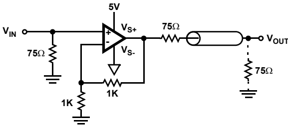
FIGURE 30. SYNC PULSE REMOVER
