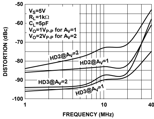
FIGURE 19. HARMONIC DISTORTION vs FREQUENCY
