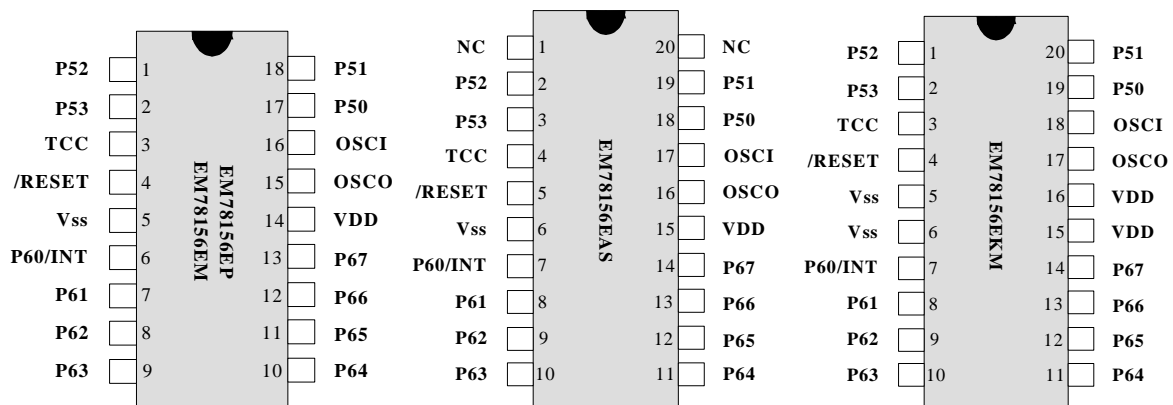
Fig. 1 Pin Assignment
