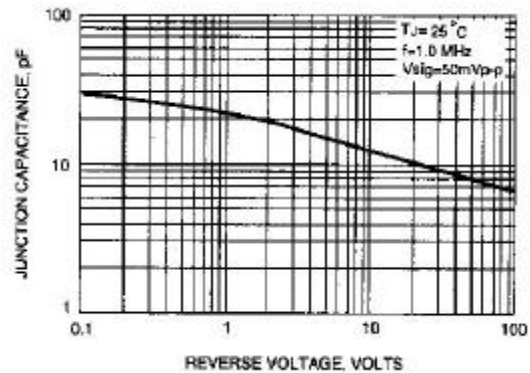
Fig. 6-TYPICAL JUNCTION CAPACITANCE
